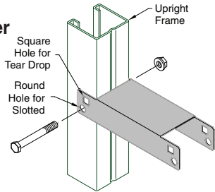
Row-to-wall Spacer
