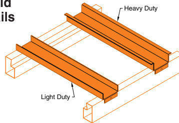
Metal Deck
