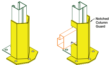
Floor Mounted
