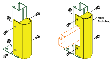
Column Mounted
