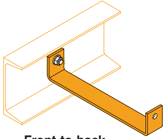
Front-to-back beam tie
